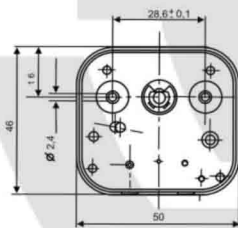
MOUNTING FOR TIMER
