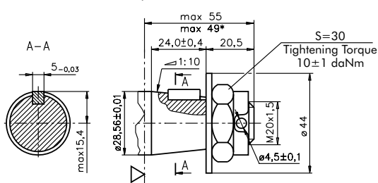
K - tapered 1:10, Parallel key B5x5x14 DIN 6885 Max. Torque 40 daNm
